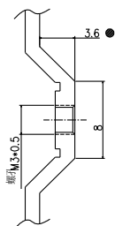
Section C-C(S:5/1) Total 2pcs "c"
