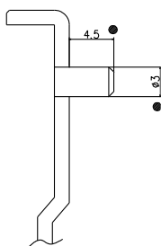
Section B-B(S: 5/1) Total 9pcs "b"
