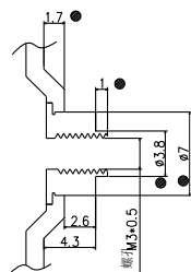
Section B-B(S: 5/1) Total 9pcs "b"
