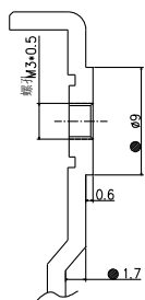
SECTION A-A (Scale: 5/1) Total 9pcs "a"
