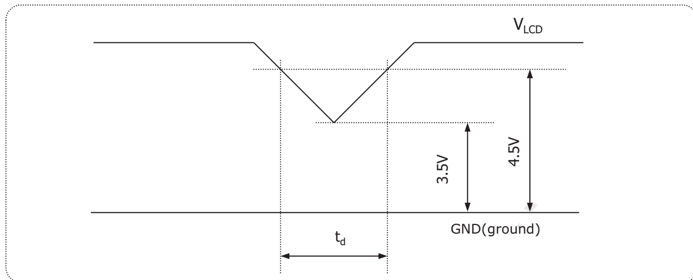
FIG.3-3 Power Dip Condition
