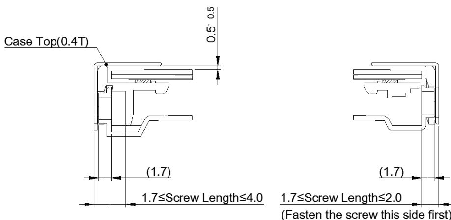
SECTION A-A SCALE 2/1
