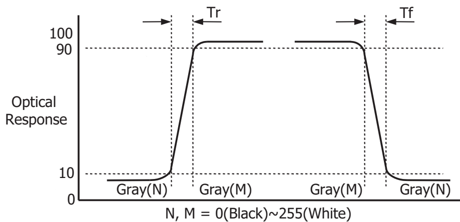
FIG.4-3 Response Time
