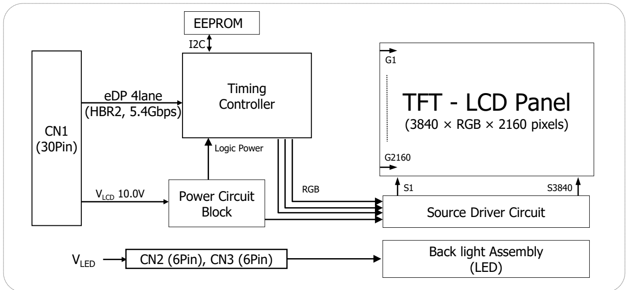
FIG.1 Block Diagram
